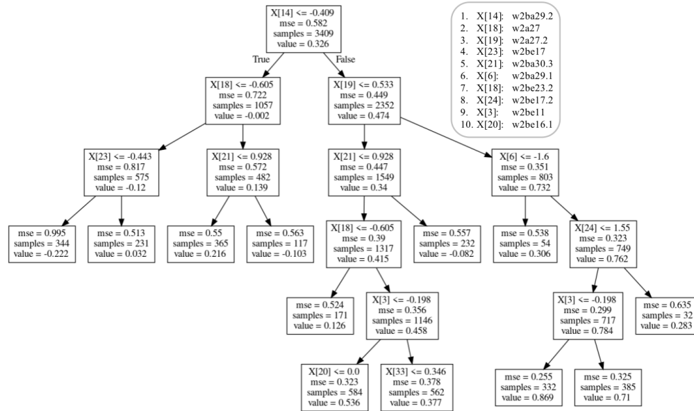
Figure 3: Regression Tree
